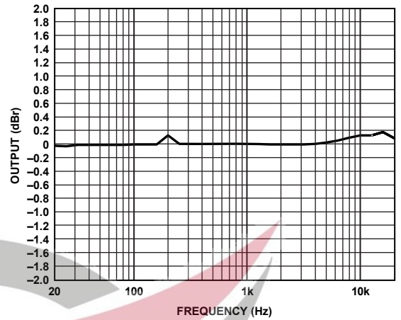
Figure 26. Frequency Response @ 1 W, 6 Ω, PVDD = 15 V, PGA = 0 dB
