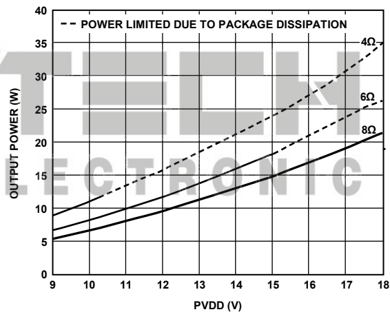
Figure 16. Output Power vs. PVDD @ 10% THD + N
