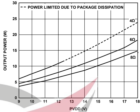
Figure 14. Output Power vs. PVDD @ 0.1% THD + N
