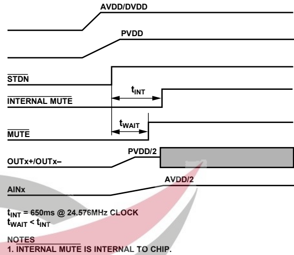
Figure 47. Power-Up Sequence, t_{WAIT} < t_{INT}
