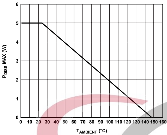
Figure 35. Power Dissipation Derating vs. Ambient Temperature
