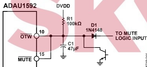
Figure 44. Option 1 Schematic for Autorecovery
