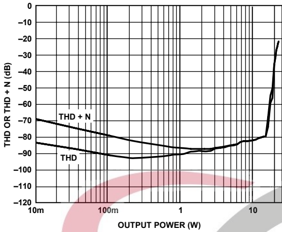
Figure 11. THD or THD + N vs. Output Power, 4 Ω, PVDD = 15 V
